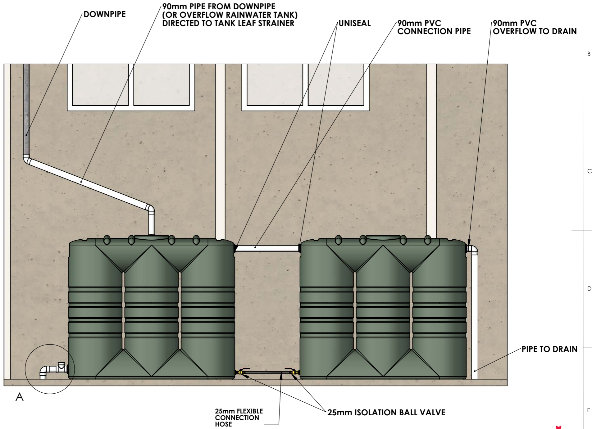
SIDE ELEVATION
